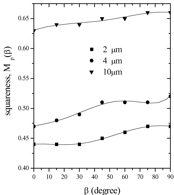
Fig. 3. Angular dependence of M_p(\beta) of the films.
