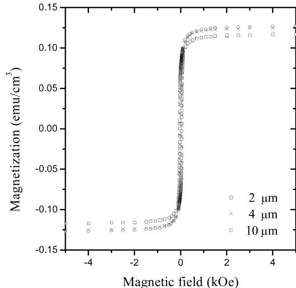
Fig. 2. Hysteresis loops of Ni-Co films measured at \beta = 0^\circ .
