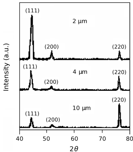
Fig. 1. XRD patterns of polycrystalline Ni-Co films.
