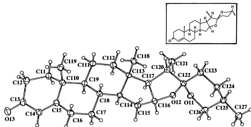
Fig. 1. Plot of one of the diosgenone molecules in the asymmetric unit showing the labeling of the non-H atoms and their displacement ellipsoids (Inset: conventional drawing of the structure).
