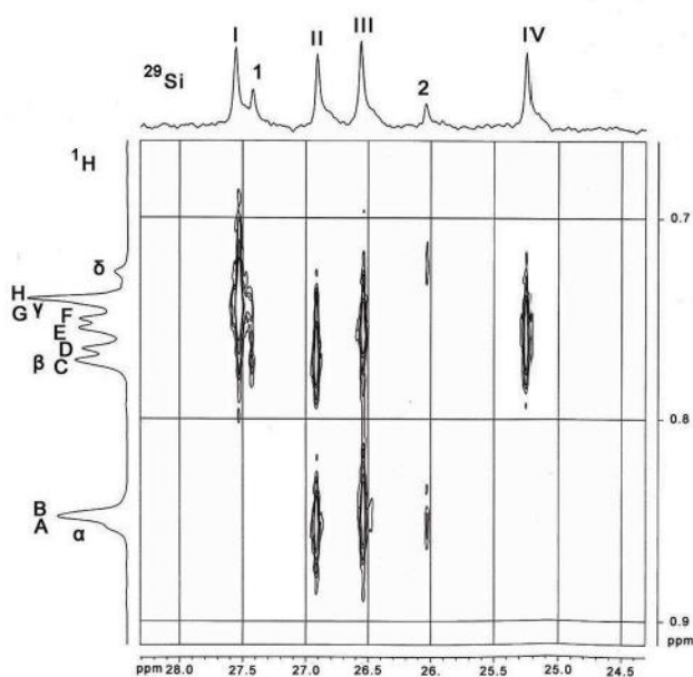
Figure S7 2D ^1\text{H}/^{29}\text{Si} NMR shift correlation spectrum of \text{C}(\text{SiClMe}_2)_4 in \text{CDCl}_3/\text{CD}_2\text{Cl}_2 at 201 K.
