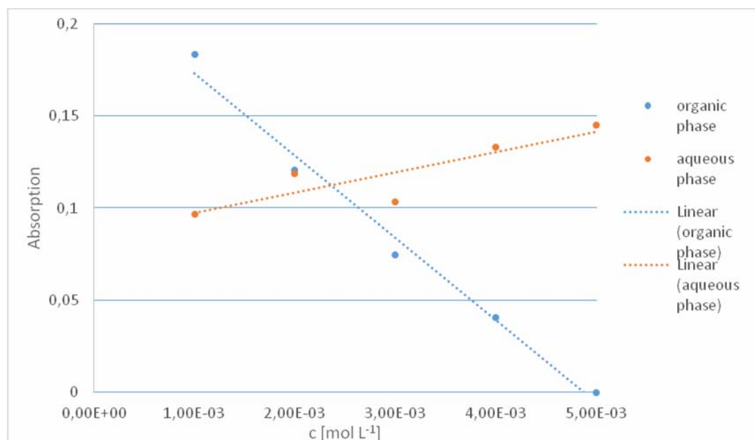
Lambert-Beer Correlation
