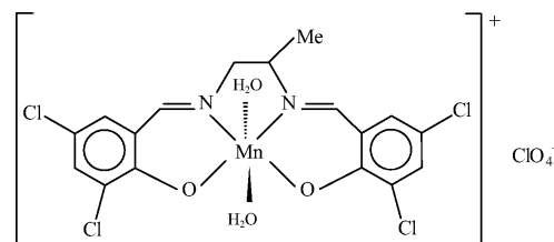
Fig. 1. Chemical structure of the title compound.
