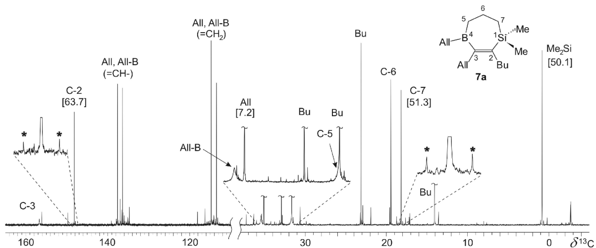
Fig. 2. 125.8 MHz ^{13}\text{C}\{^1\text{H}\} NMR spectrum of the reaction mixture after conversion of the alkene 5a into the seven-member heterocycle 7a . Note the typically broad and weak ^{13}\text{C} NMR signals for the carbon atoms linked to boron [18] and the satellites owing to J(^{29}\text{Si}, ^{13}\text{C}) (data in Hz given in brackets).
