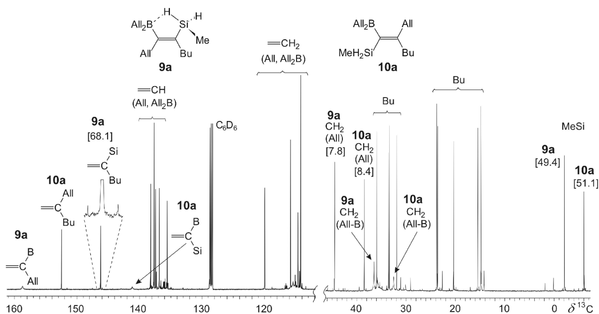
Fig. 3. 125.8 MHz ^{13}\text{C}\{^1\text{H}\} NMR spectrum of the reaction mixture containing the alkenes 9a and 10a formed by 1,1- and 1,2-allylboration, respectively, of the alkyne 3a . A small amount of an excess of triallylborane is still present. Note the typically broad and weak ^{13}\text{C} NMR signals for the carbon atoms linked to boron [18] and the satellites owing to J(^{29}\text{Si}, ^{13}\text{C}) (data in Hz given in brackets).
