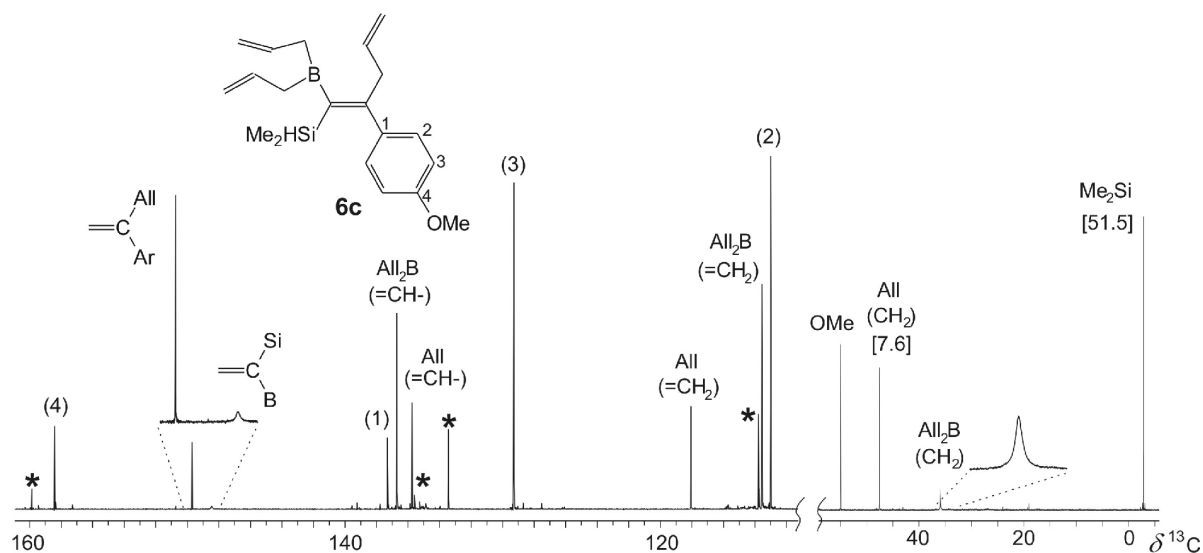
Fig. 1. 125.8 MHz ^{13}\text{C}\{^1\text{H}\} NMR spectrum of the reaction mixture containing the alkene 6c , formed selectively by 1,2-allylboration, together with a small amount of unreacted 3c (signals marked by asterisks). Note the typically broad and weak ^{13}\text{C} NMR signals for the carbon atoms linked to boron [18] and the satellites owing to J(^{29}\text{Si}, ^{13}\text{C}) (data in Hz given in brackets).
