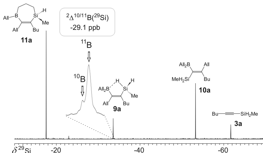
Fig. 4. 99.6 MHz ^{29}\text{Si}\{^1\text{H}\} NMR spectrum of the reaction mixture containing a small amount of the starting alkyne 3a , the products of 1,1- and 1,2-allylboration 9a and 10a , respectively, as well as the seven-member heterocycle 11a , formed by intramolecular hydrosilylation of 9a . The isotope-induced chemical shift ^2\Delta^{10/11}\text{B}(^{29}\text{Si}) , is typical of the Si-H-B bridge in 9a .
