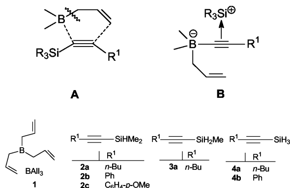
Scheme 1. Alkyn-1-ylsilanes employed in the reaction with triallylborane.
