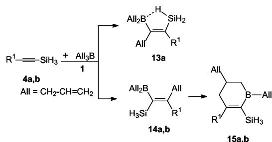
Scheme 5. Allylboration of alkyn-1-yl(trihydrido)silanes.
