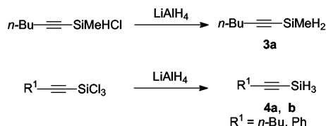
Scheme 2. Reduction of alkyn-1-yl(chloro)silanes with \text{LiAlH}_4 .
