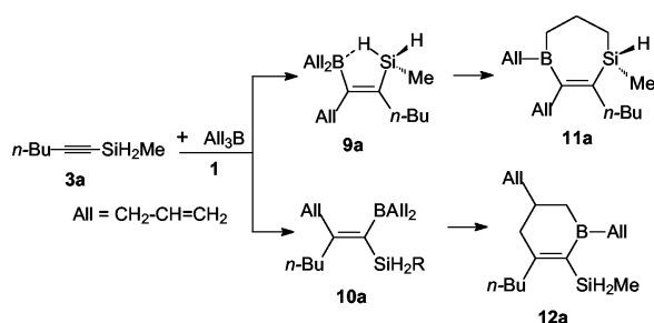
Scheme 4. Allylboration of alkynyl-(dihydrido)silanes.
