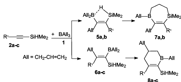
Scheme 3. Allylboration of alkyn-1-yl(hydrido)silanes.
