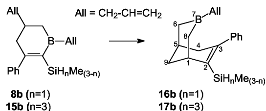
Scheme 6. Rearrangement of 1-bora-cyclohexa-2-enes into 7-borabicyclo[3.3.1]non-2-enes.
